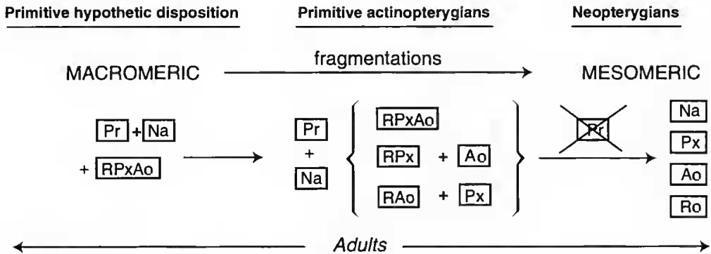
Fig. 3. — Hypothesis about the evolution of the dermal snout after Pehrson (1947, 1958), Gardiner (1963, 1984), Jessen (1968), and others (see text). Ao, antorbital; APx, antorbito-premaxillary; Na, nasal; Px, premaxillary; Pr, postrostral; RAo, rostro-antorbital; Ro, rostral; RPx, rostro-premaxillary; RPxAo, rostro-premaxillo-antorbital; RPr, rostro-postrostral.
